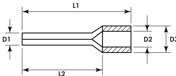
DIMENSIONS (mm)
